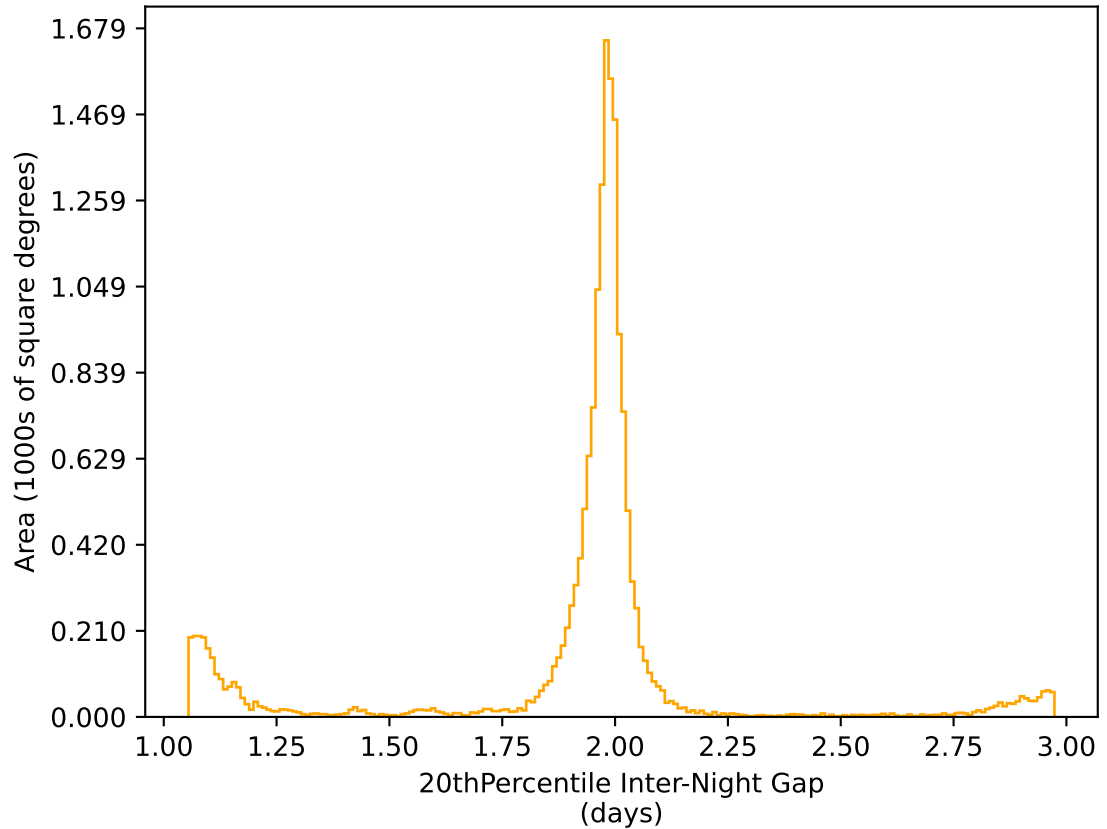
ddf_acor_sf10_lsf15_lsr20_v3.4_10yrs WFD r band: 20thPercentile Inter-Night Gap
