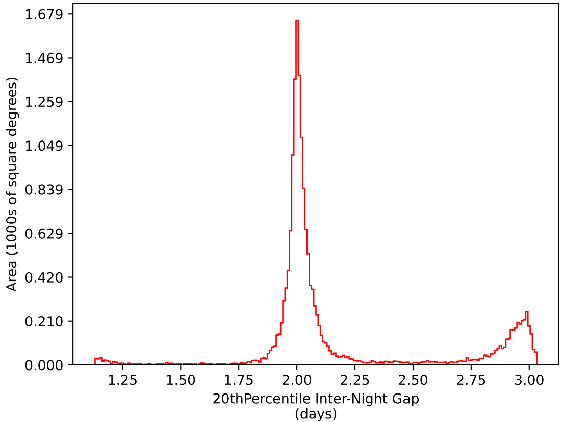
ddf_acor_sf10_lsf15_lsr20_v3.4_10yrs WFD i band: 20thPercentile Inter-Night Gap
