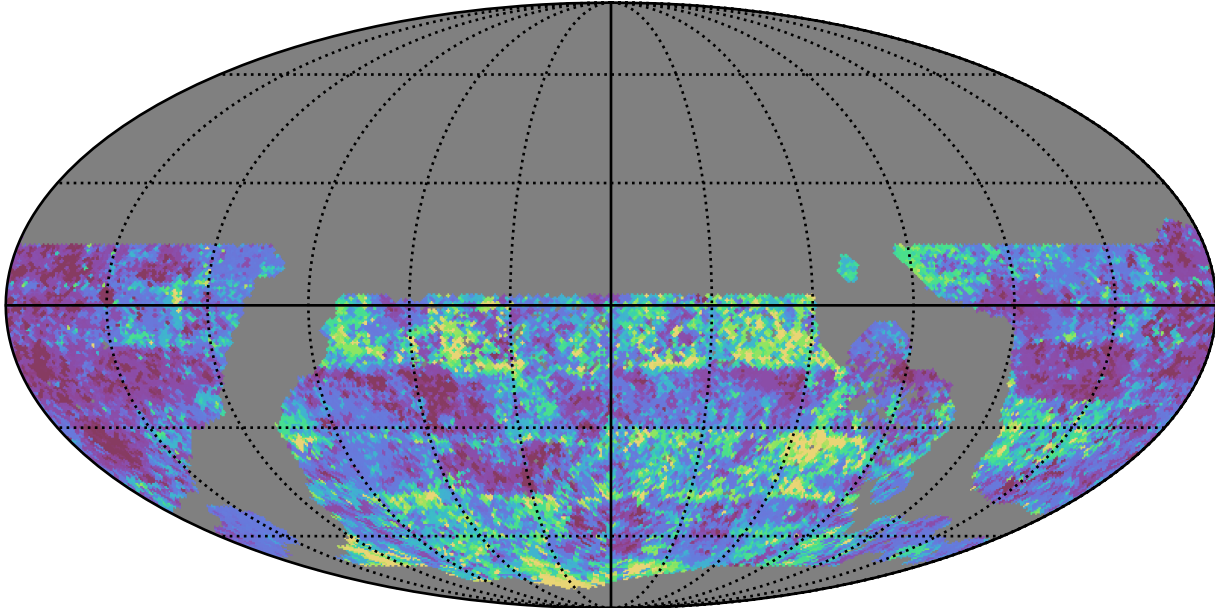
ddf_acor_sf10_lsf15_lsr20_v3.4_10yrs WFD g band: 20thPercentile Inter-Night Gap
