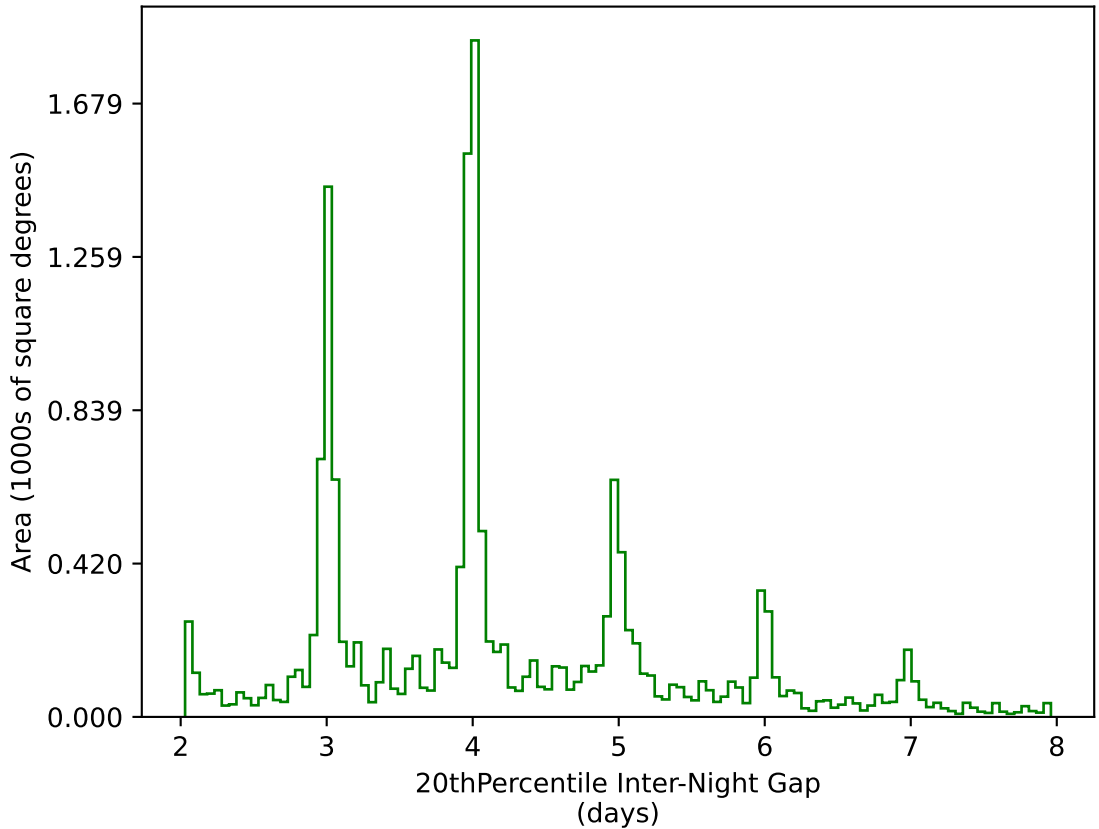
ddf_acor_sf10_ls15_lsr20_v3.4_10yrs WFD g band: 20thPercentile Inter-Night Gap
