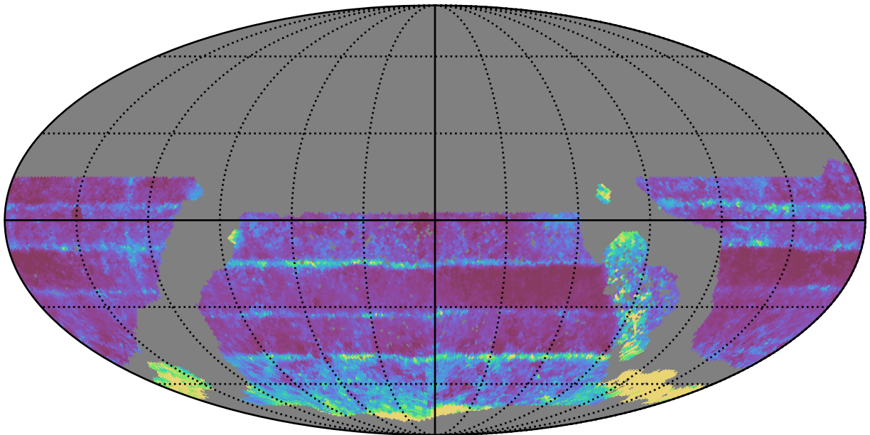
ddf_acor_sf10_lsf15_lsr20_v3.4_10yrs WFD all bands: 20thPercentile Inter-Night Gap
