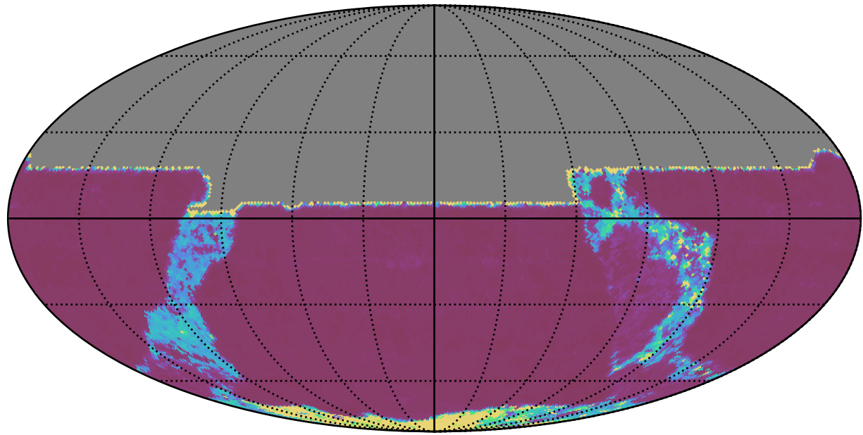
ddf_acor_sf10_lsf15_lsr20_v3.4_10yrs All sky y band: 20thPercentile Inter-Night Gap
