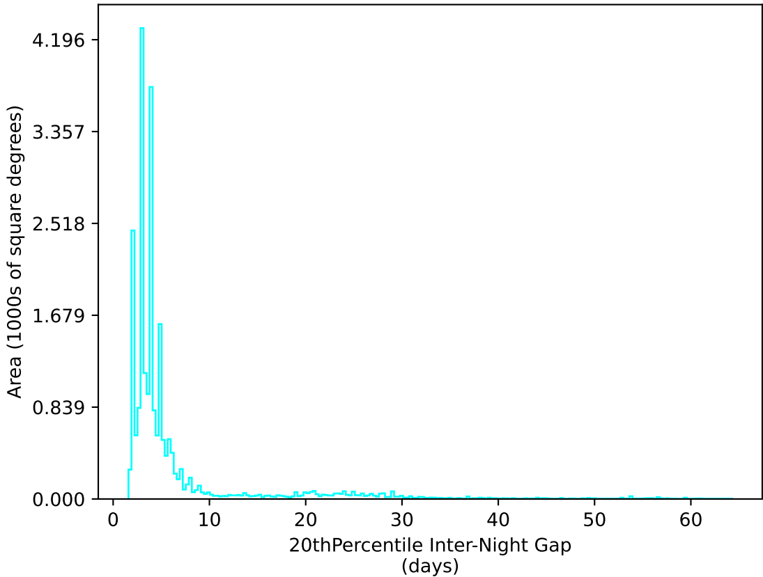
ddf_acor_sf10_ls15_lsr20_v3.4_10yrs All sky u band: 20thPercentile Inter-Night Gap
