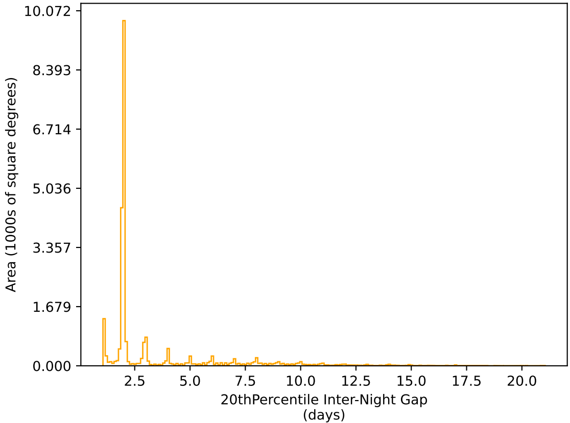
ddf_acor_sf10_ls15_lsr20_v3.4_10yrs All sky r band: 20thPercentile Inter-Night Gap
