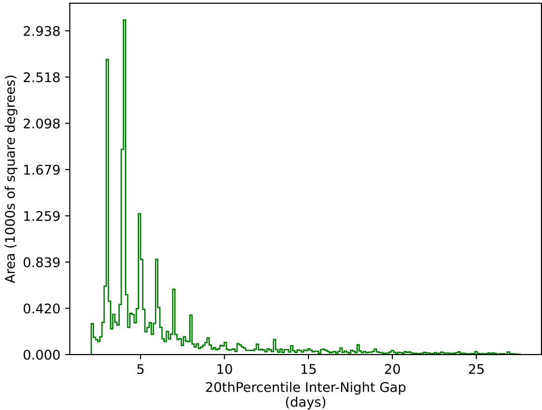
ddf_acor_sf10_ls15_lsr20_v3.4_10yrs All sky g band: 20thPercentile Inter-Night Gap
