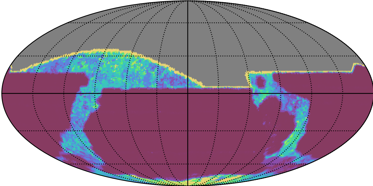
ddf_acor_sf10_lsf15_lsr20_v3.4_10yrs All sky all bands: 20thPercentile Inter-Night Gap
