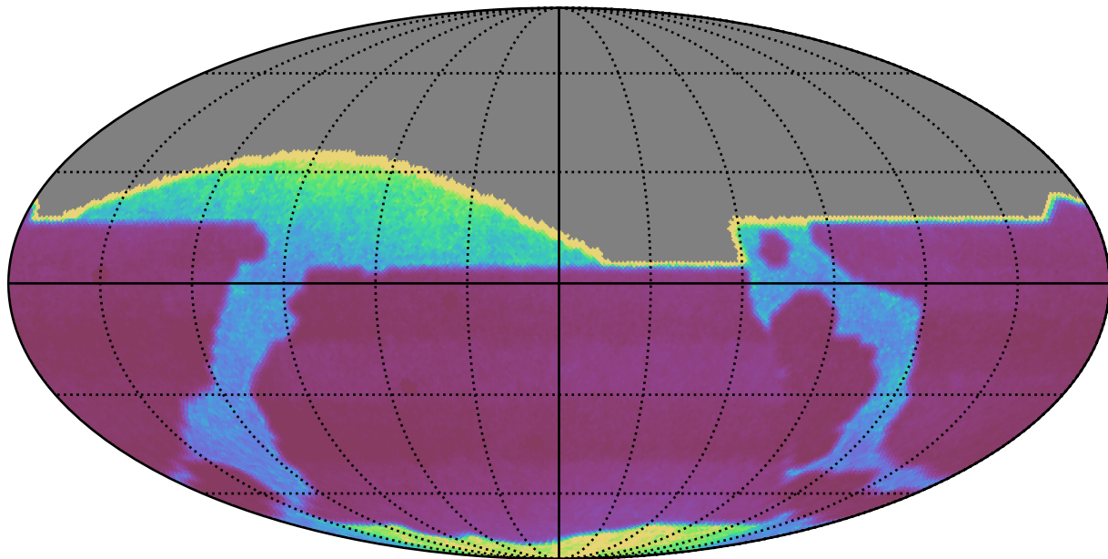
ddf_acor_sf10_lsf15_lsr20_v3.4_10yrs : properMotion
