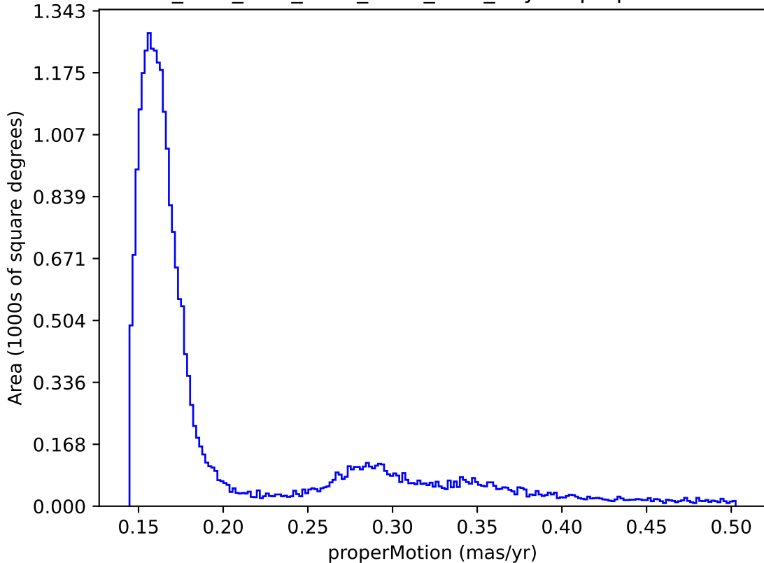
ddf_acor_sf10_ls15_lsr20_v3.4_10yrs : properMotion
