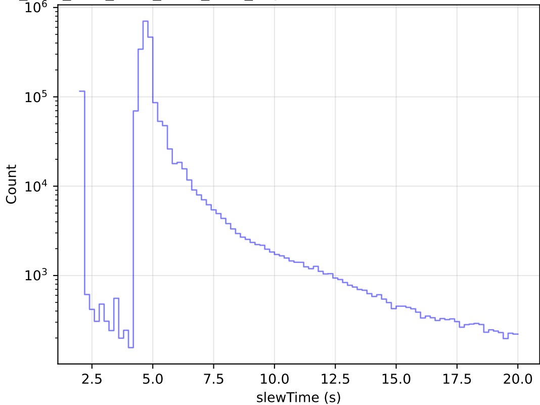
ddf_acor_sf10_lsf15_lsr20_v3.4_10yrs All visits: Zoom Slew Time Histogram
