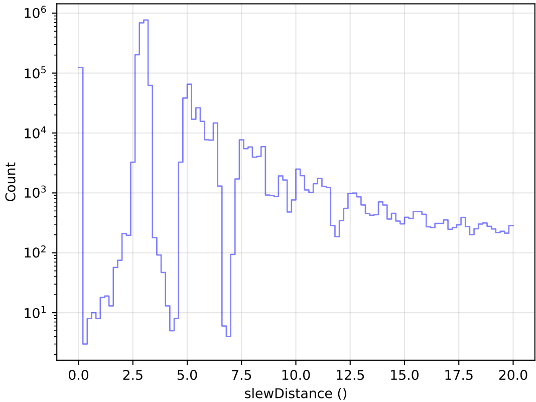
ddf_acor_sf10_lsf15_lsr20_v3.4_10yrs All visits: Zoom Slew Distance Histogram
