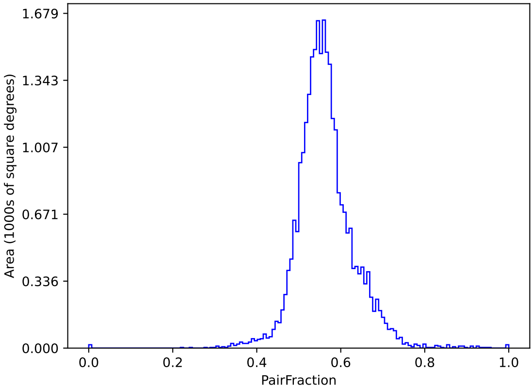
ddf_acor_sf10_lsf15_lsr20_v3.4_10yrs (g or r or i): PairFraction
