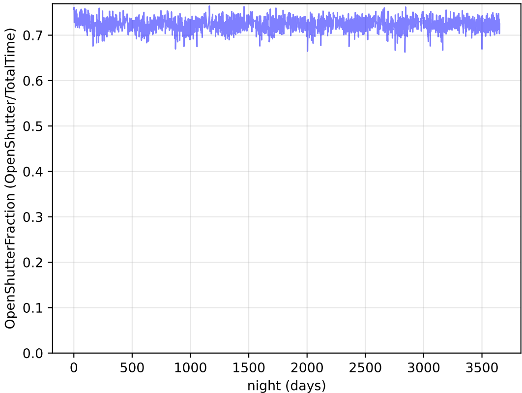
ddf_acor_sf10_lsf15_lsr20_v3.4_10yrs : OpenShutterFraction
