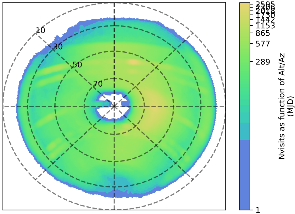
ddf_acor_sf10_lsf15_lsr20_v3.4_10yrs z: Nvisits as function of Alt/Az
