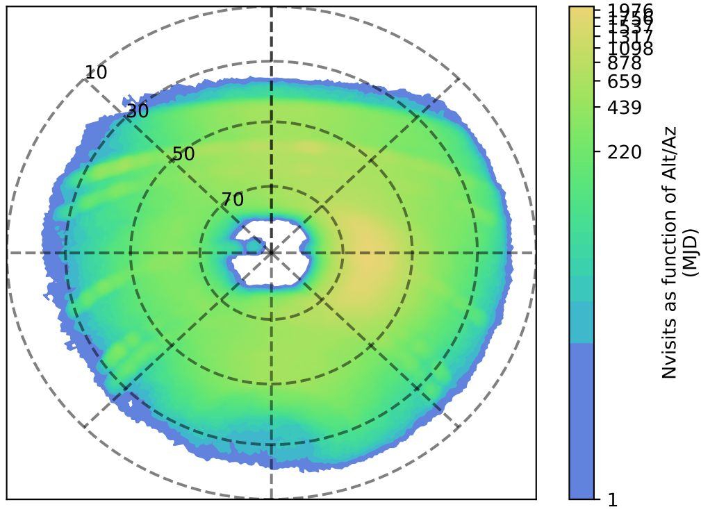
ddf_acor_sf10_ls15_lsr20_v3.4_10yrs y: Nvisits as function of Alt/Az
