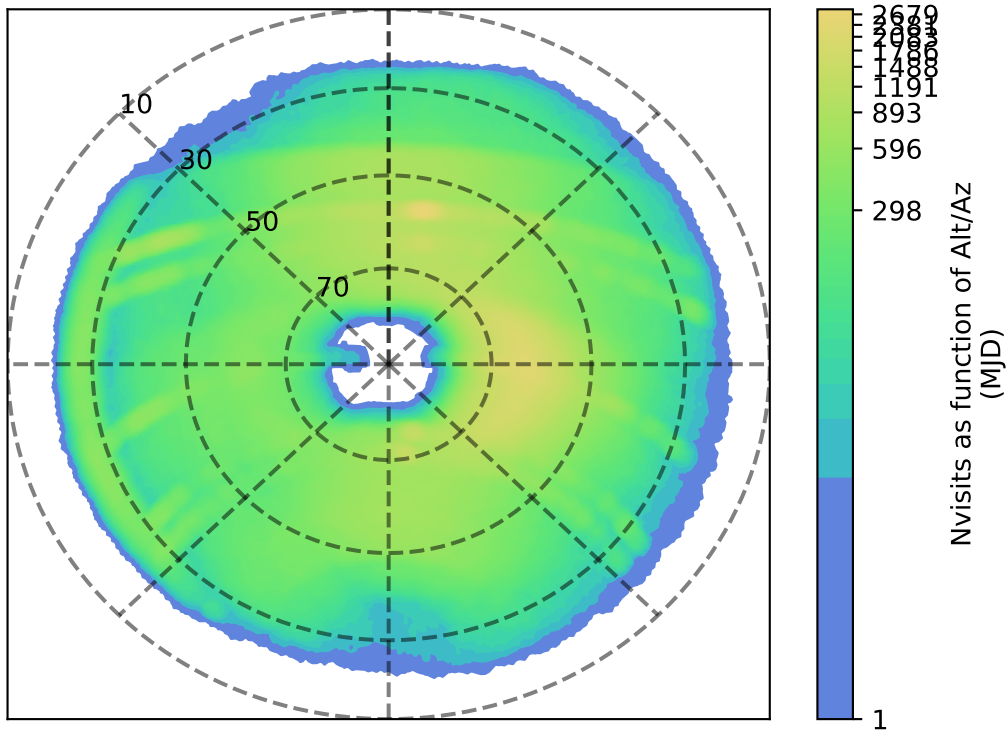
ddf_acor_sf10_ls15_lsr20_v3.4_10yrs r: Nvisits as function of Alt/Az
