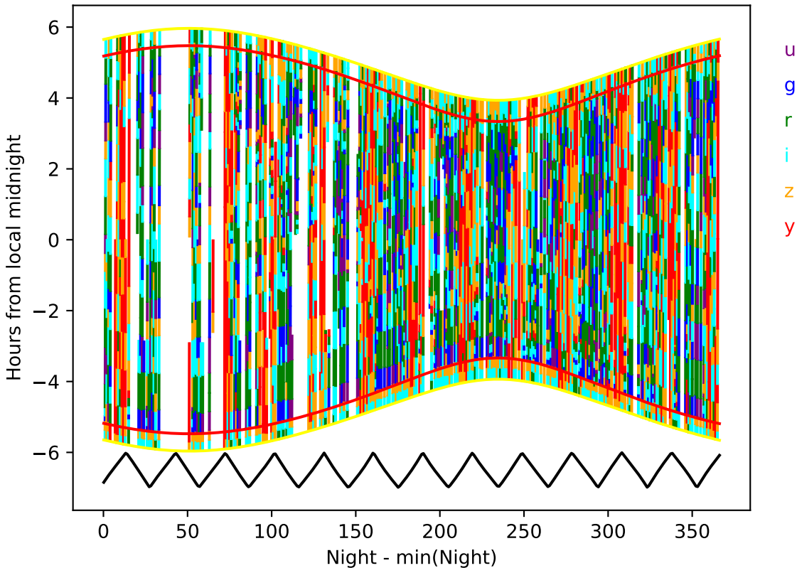
ddf_acor_sf10_lsf15_lsr20_v3.4_10yrs year 8-9: Hourglass
