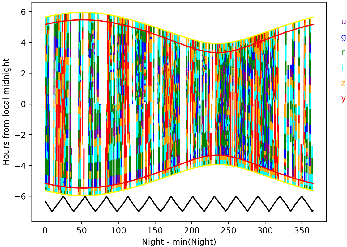
ddf_acor_sf10_ls15_lsr20_v3.4_10yrs year 7-8: Hourglass
