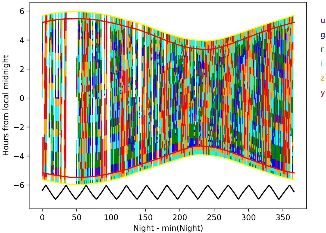
ddf_acor_sf10_lsf15_lsr20_v3.4_10yrs year 6-7: Hourglass
