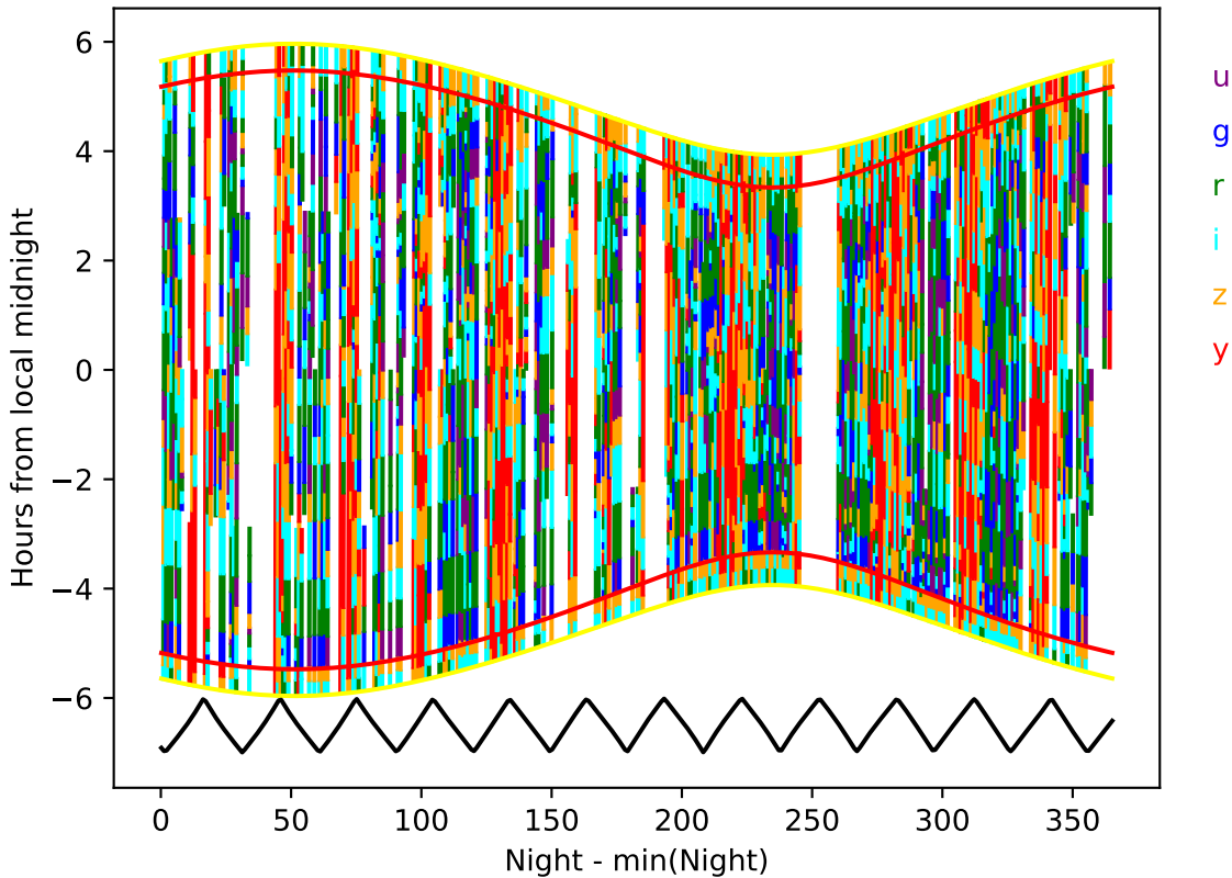
ddf_acor_sf10_ls15_lsr20_v3.4_10yrs year 5-6: Hourglass
