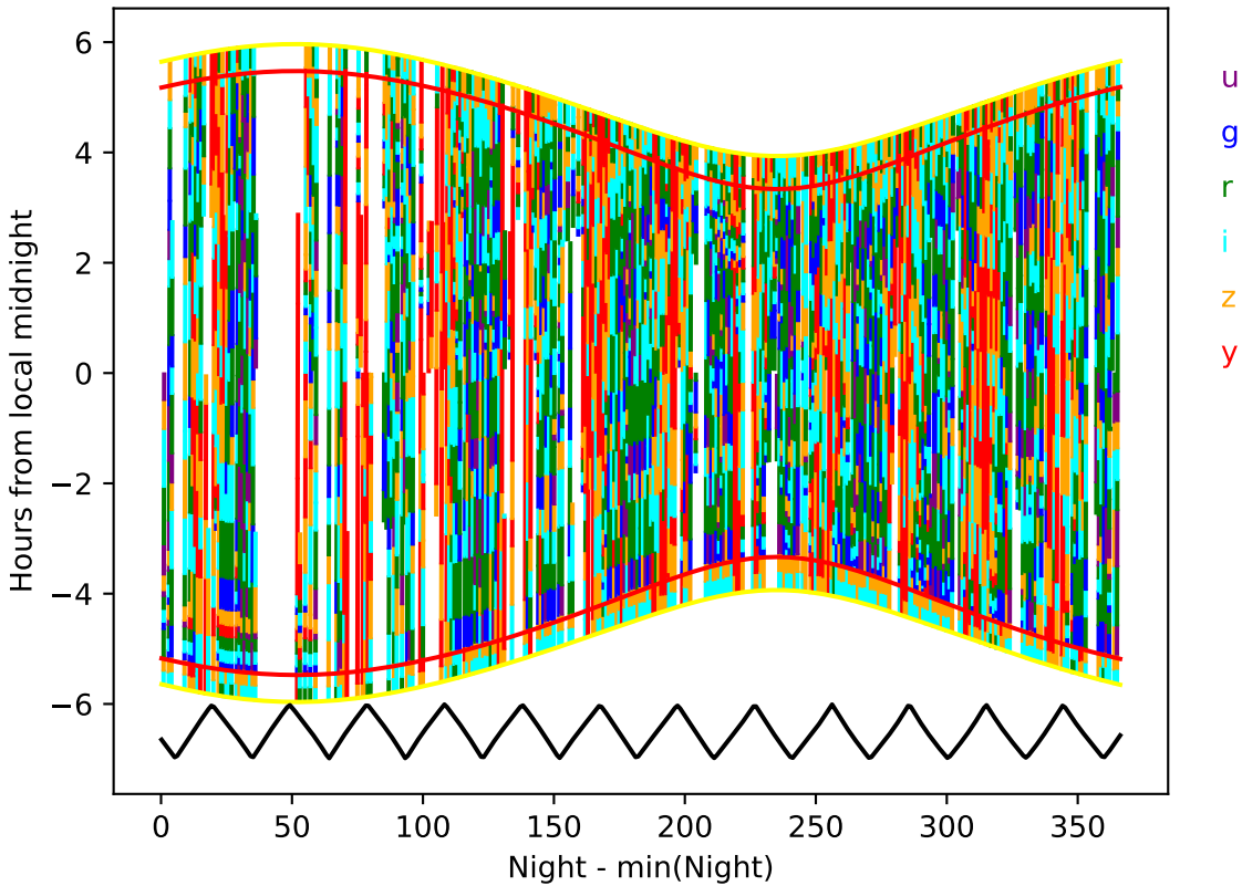
ddf_acor_sf10_ls15_lsr20_v3.4_10yrs year 2-3: Hourglass
