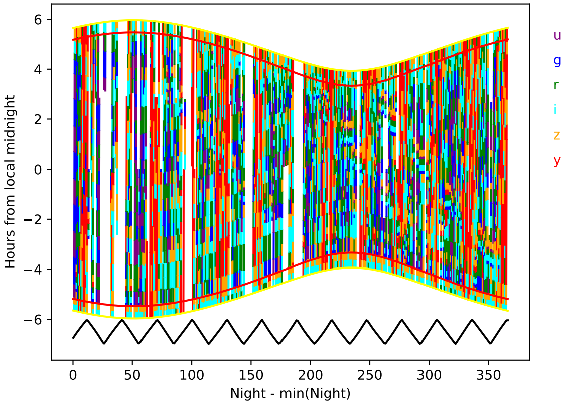
ddf_acor_sf10_lsf15_lsr20_v3.4_10yrs year 0-1: Hourglass
