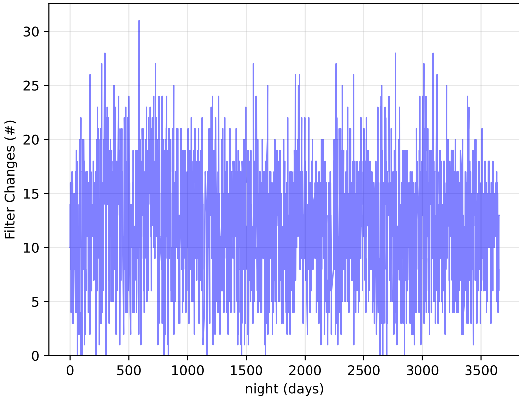
ddf_acor_sf10_lsf15_lsr20_v3.4_10yrs : Filter Changes
