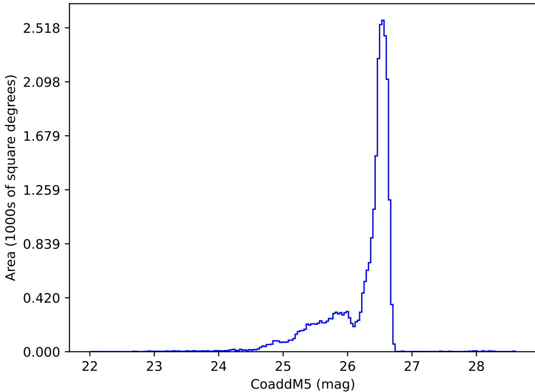
ddf_acor_sf10_lsf15_lsr20_v3.4_10yrs i: CoaddM5
