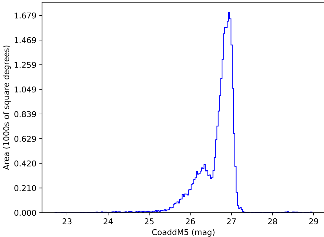
ddf_acor_sf10_ls15_lsr20_v3.4_10yrs g: CoaddM5
