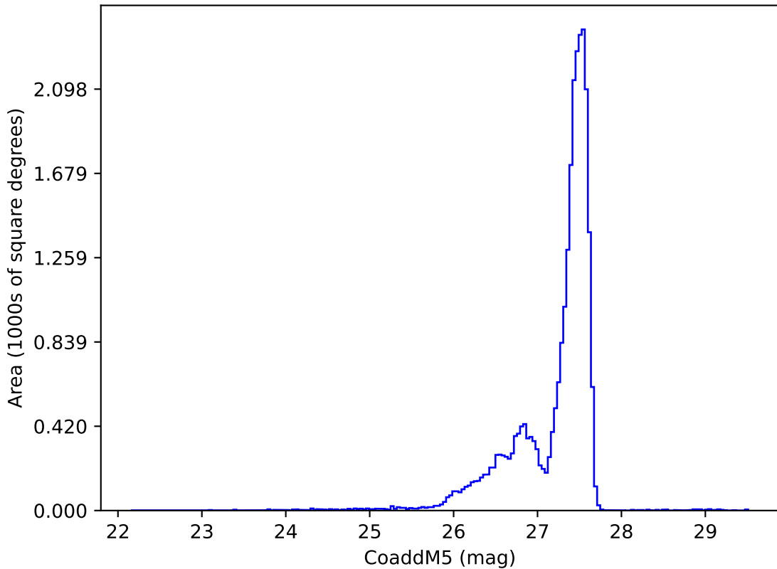
ddf_acor_sf10_lsf15_lsr20_v3.4_10yrs : CoaddM5
