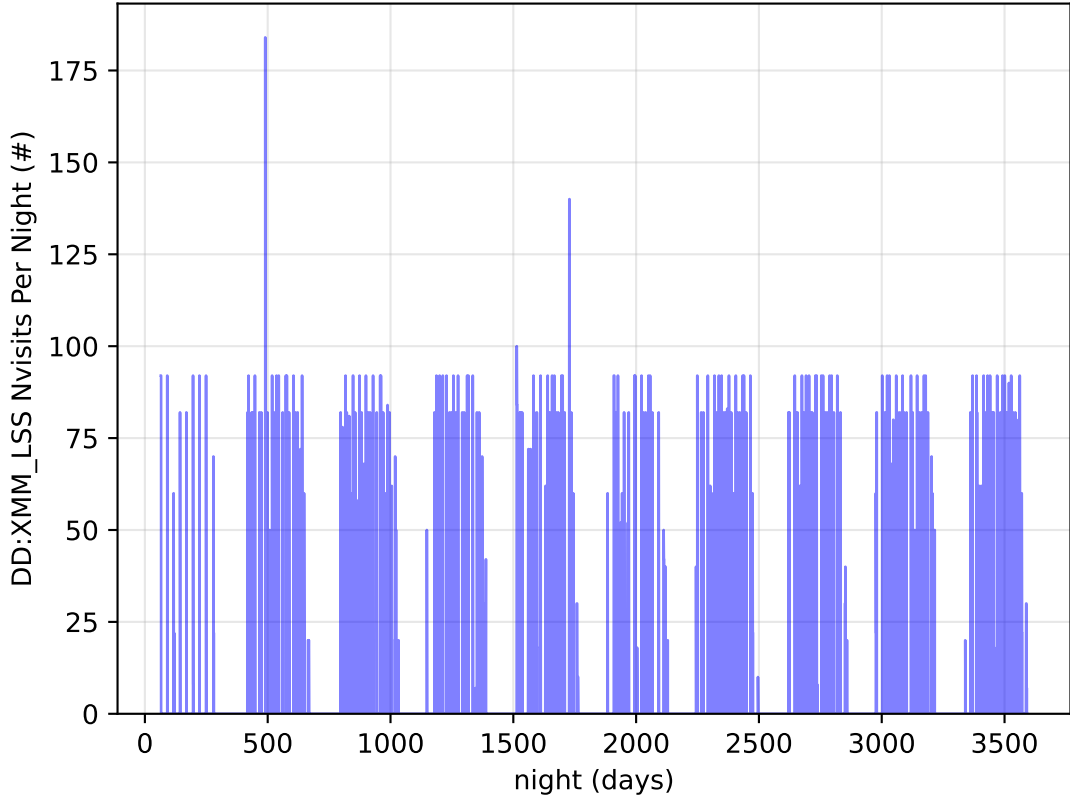
ddf_acor_sf10_lsf15_lsr20_v3.4_10yrs all bands: DD:XMM_LSS Nvisits Per Night
