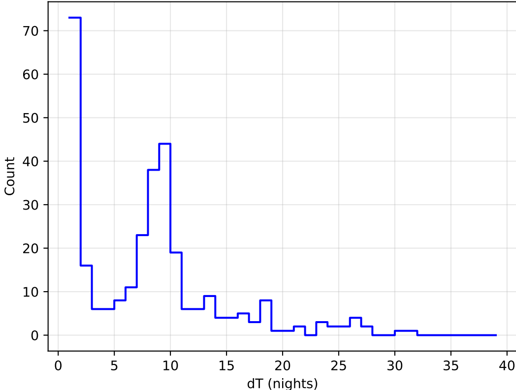
ddf_acor_sf10_lsf15_lsr20_v3.4_10yrs all bands: DD:XMM_LSS Delta Nights Histogram
