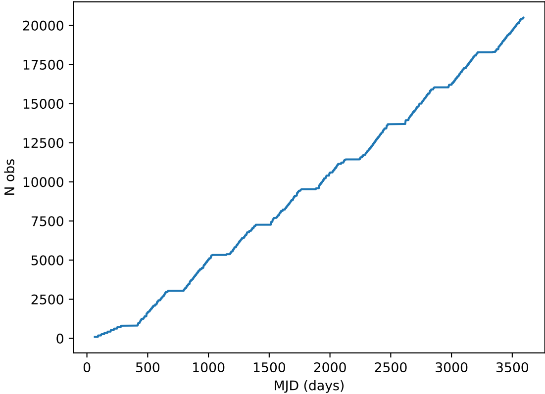
ddf_acor_sf10_lsf15_lsr20_v3.4_10yrs all bands: DD:XMM_LSS Cumulative NVisits
