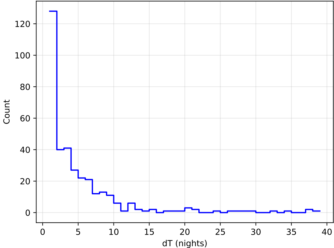
ddf_acor_sf10_lsf15_lsr20_v3.4_10yrs all bands: DD:WFD Delta Nights Histogram
