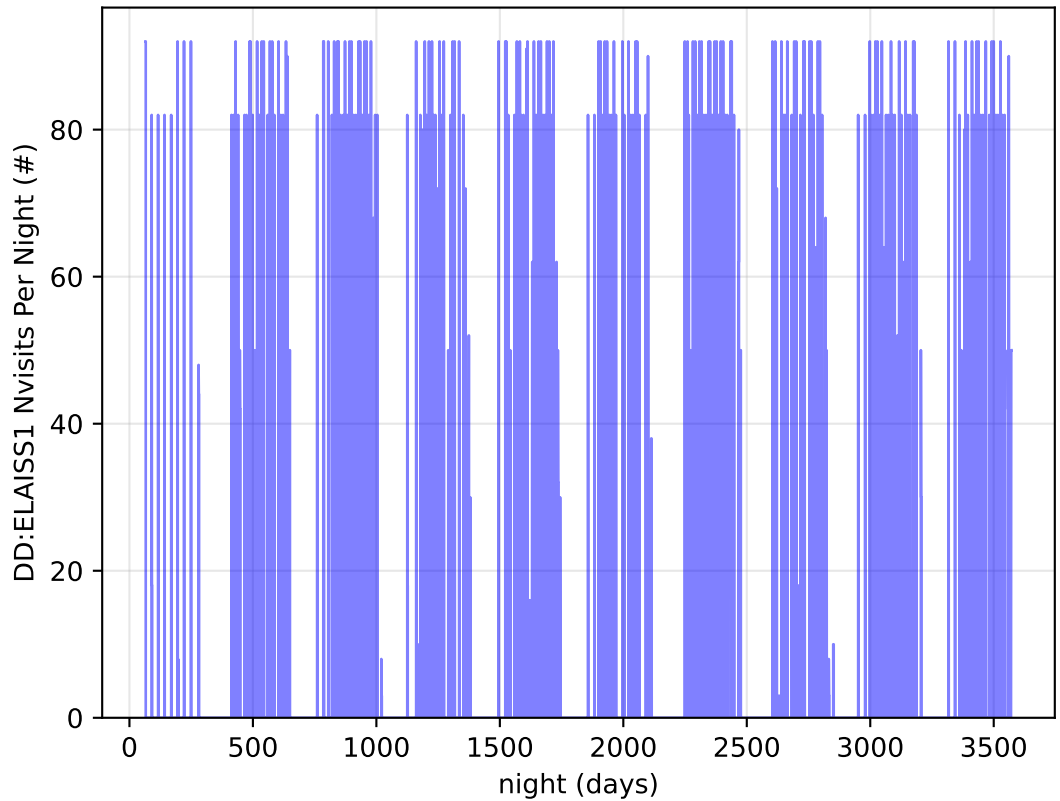
ddf_acor_sf10_lsf15_lsr20_v3.4_10yrs all bands: DD:ELAISS1 Nvisits Per Night
