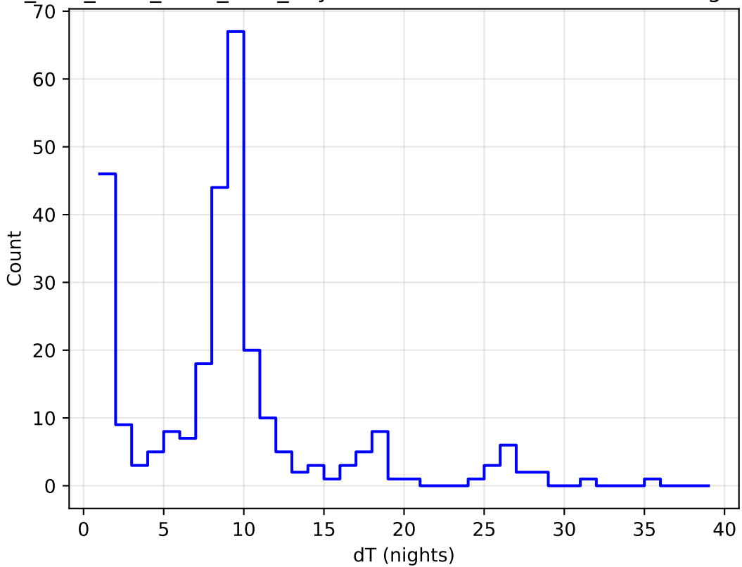
ddf_acor_sf10_lsf15_lsr20_v3.4_10yrs all bands: DD:ELAISS1 Delta Nights Histogram
