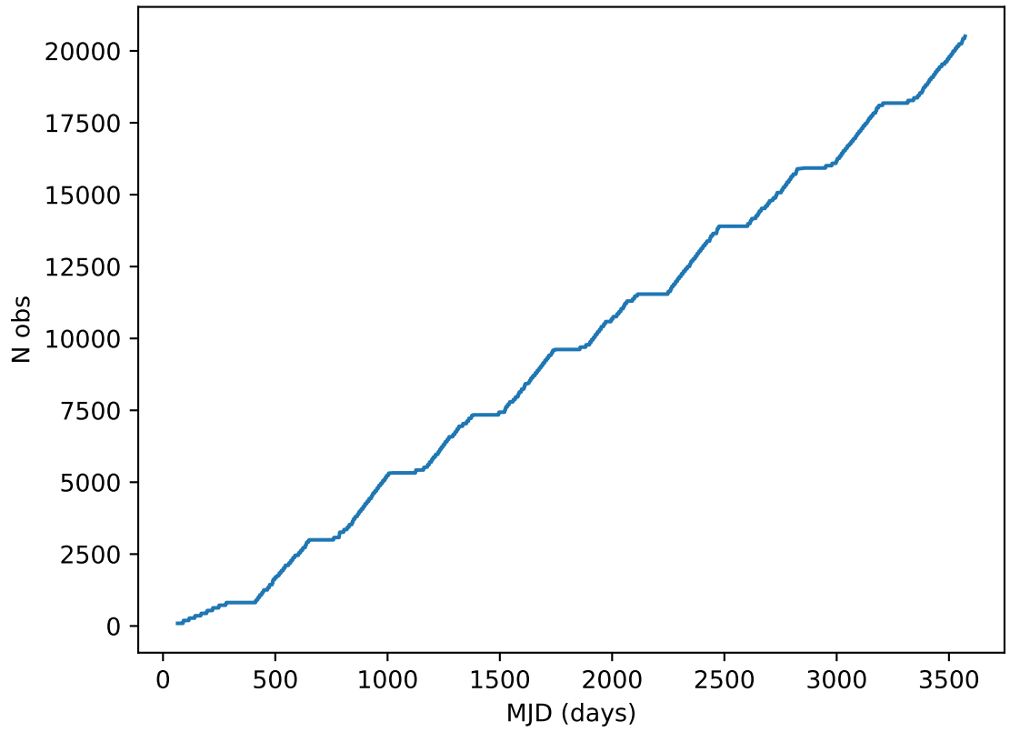
ddf_acor_sf10_lsf15_lsr20_v3.4_10yrs all bands: DD:ELAISS1 Cumulative NVisits
