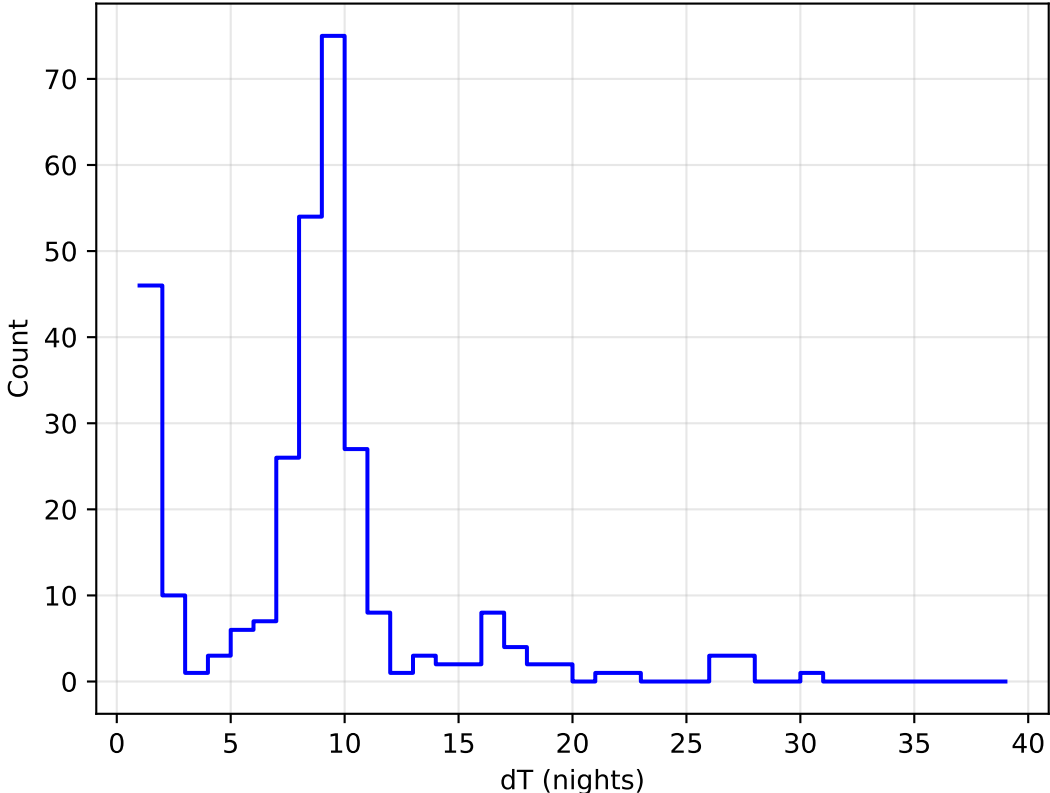
ddf_acor_sf10_lsf15_lsr20_v3.4_10yrs all bands: DD:EDFS Delta Nights Histogram
