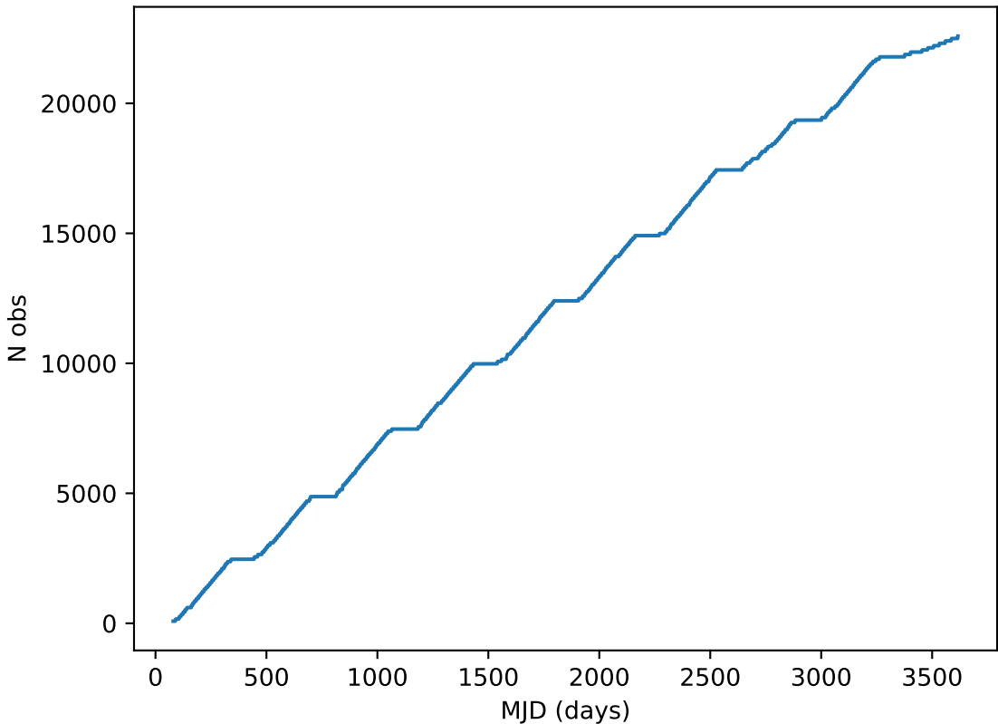
ddf_acor_sf10_lsf15_lsr20_v3.4_10yrs all bands: DD:EDFS Cumulative NVisits
