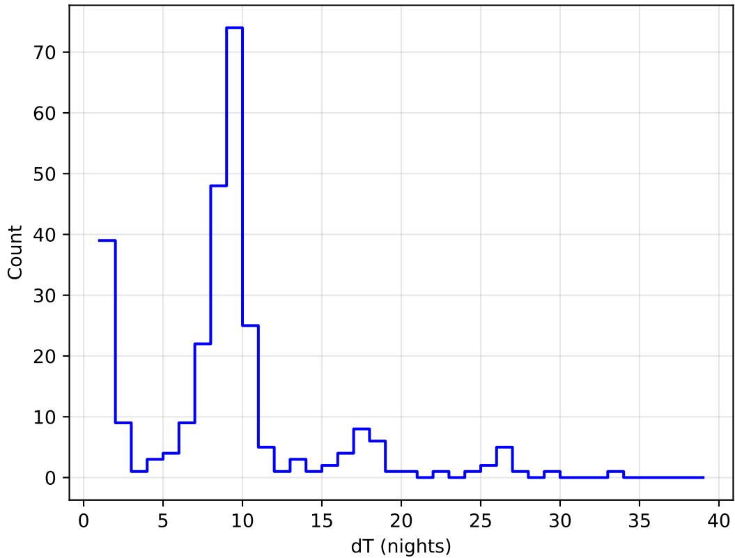
ddf_acor_sf10_lsf15_lsr20_v3.4_10yrs all bands: DD:ECDFS Delta Nights Histogram
