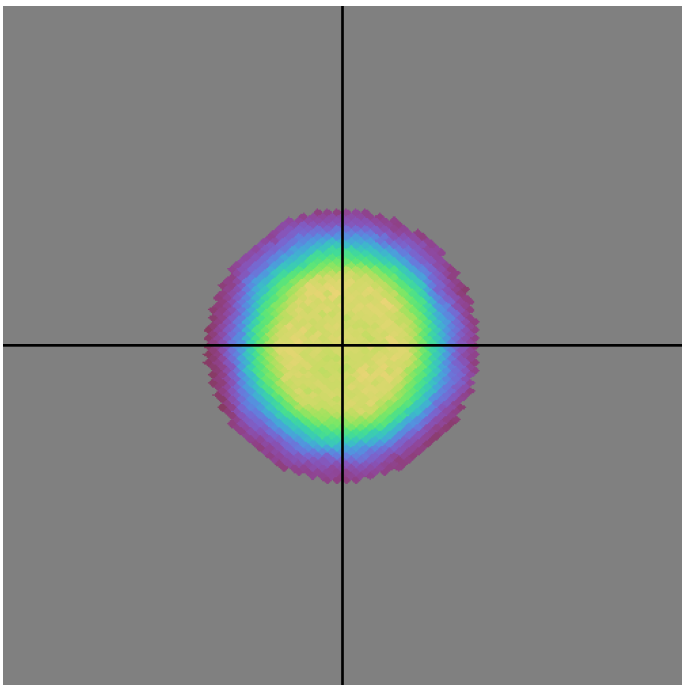
ddf_acor_sf10_lsf15_lsr20_v3.4_10yrs all bands: DD:COSMOS N Unique Nights
