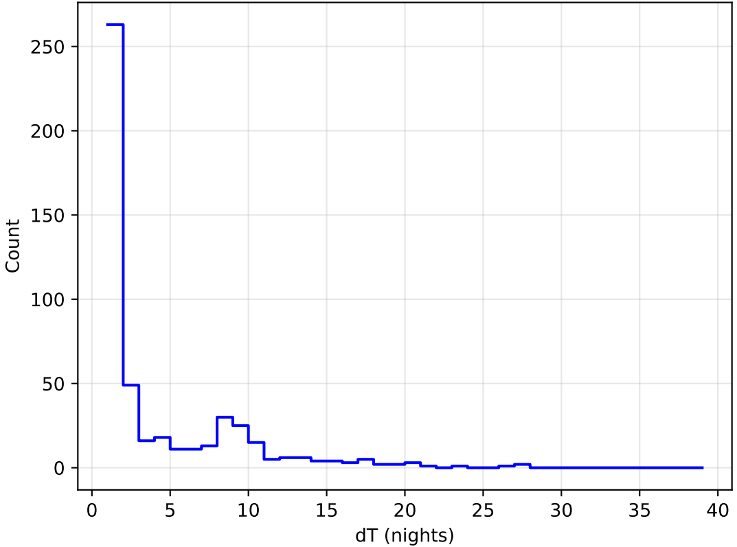
ddf_acor_sf10_Isf15_Isr20_v3.4_10yrs all bands: DD: COSMOS Delta Nights Histogram
