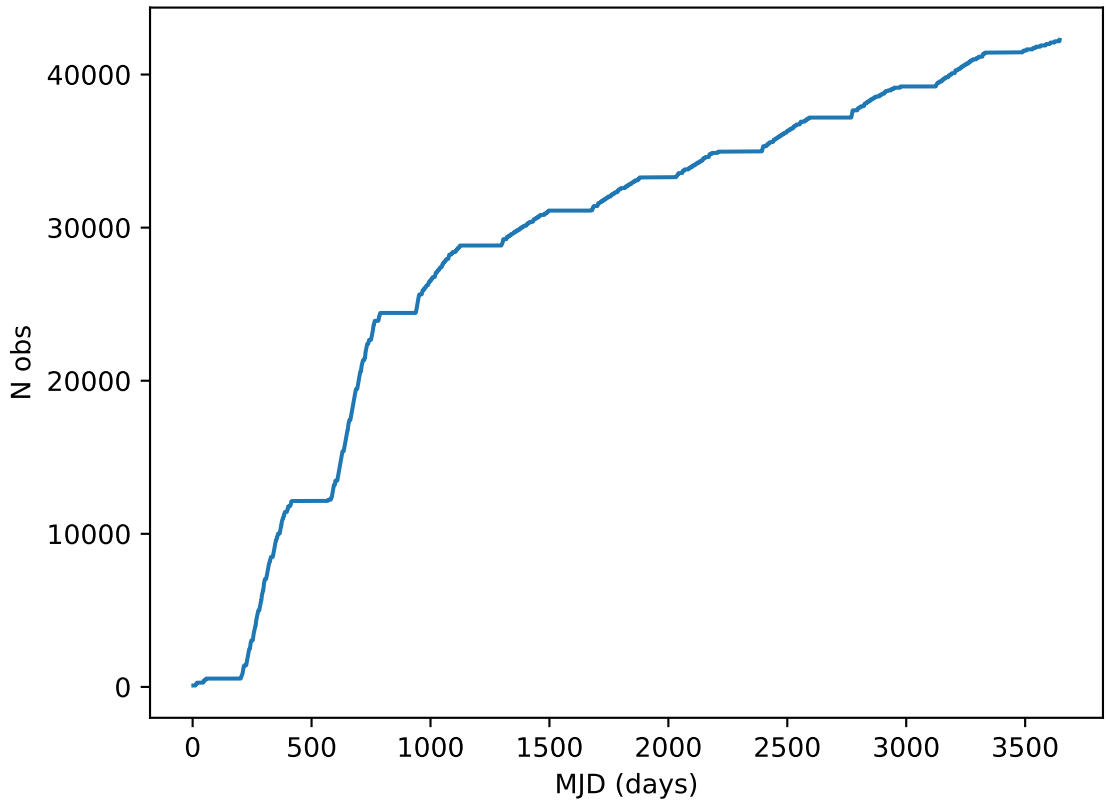
ddf_acor_sf10_lsf15_lsr20_v3.4_10yrs all bands: DD: COSMOS Cumulative NVisits
