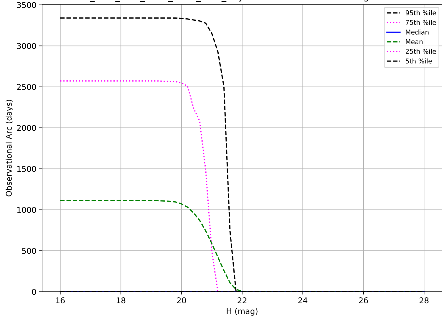
ddf_acor_sf10_lsf15_lsr10_v3.4_10yrs: Observational Arc Length Vatira
