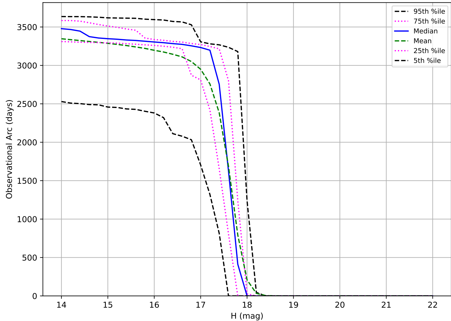
ddf_acor_sf10_lsf15_lsr10_v3.4_10yrs: Observational Arc Length Trojan
