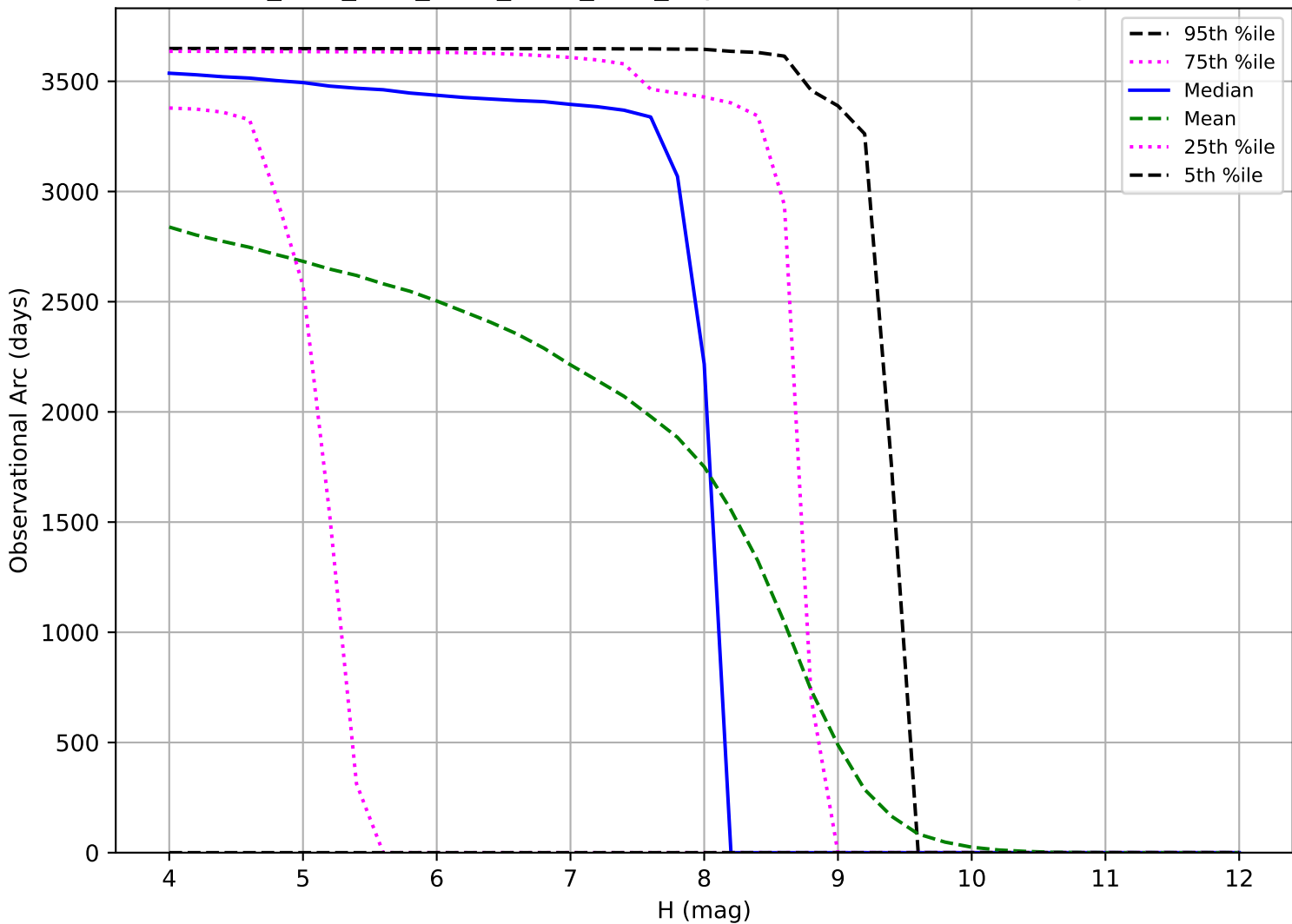
ddf_acor_sf10_lsf15_lsr10_v3.4_10yrs: Observational Arc Length TNO
