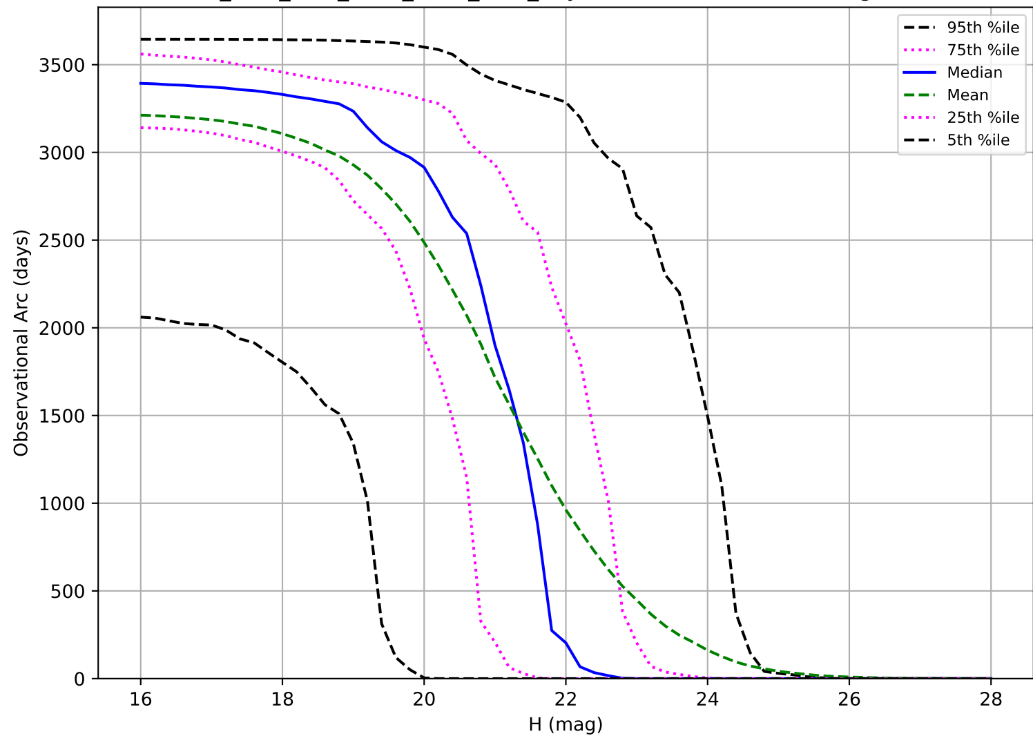
ddf_acor_sf10_lsf15_lsr10_v3.4_10yrs: Observational Arc Length PHA
