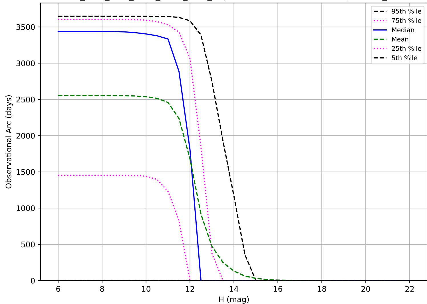
ddf_acor_sf10_lsf15_lsr10_v3.4_10yrs: Observational Arc Length OCC_r20
