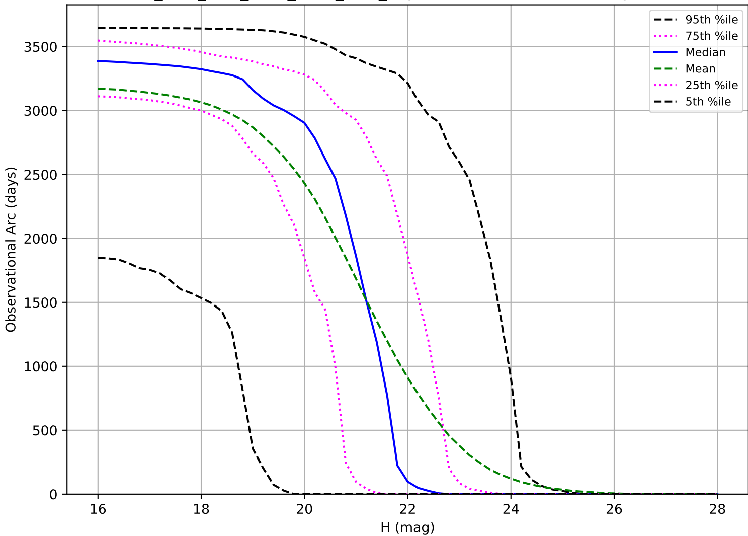
ddf_acor_sf10_lsf15_lsr10_v3.4_10yrs: Observational Arc Length NEO
