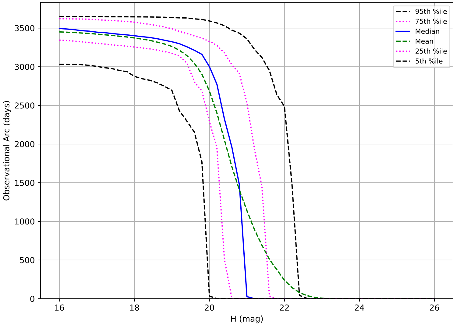
ddf_acor_sf10_lsf15_lsr10_v3.4_10yrs: Observational Arc Length MBA
