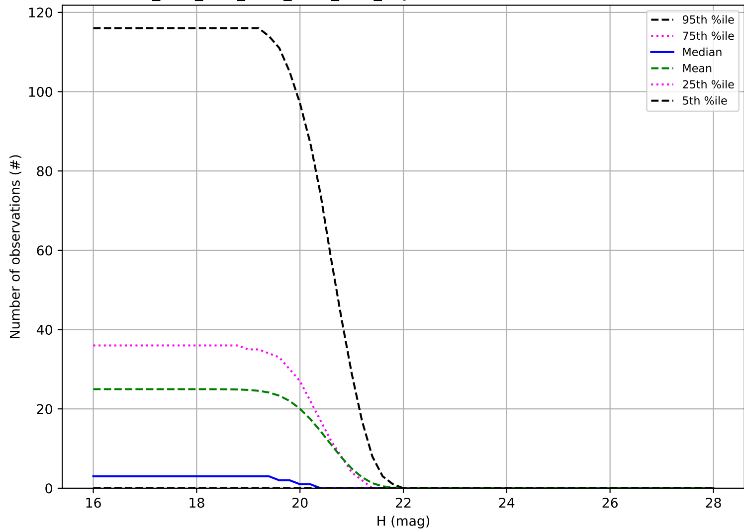
ddf_acor_sf10_lsf15_lsr10_v3.4_10yrs: Number of observations Vatira
